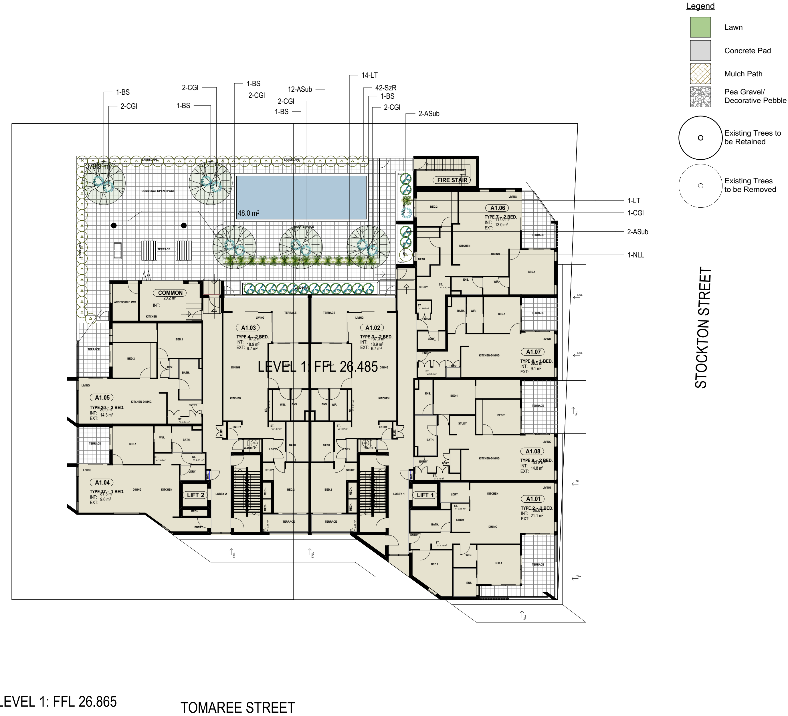
LANDSCAPE PLAN- FIRST FLOOR Scale: 1:200
